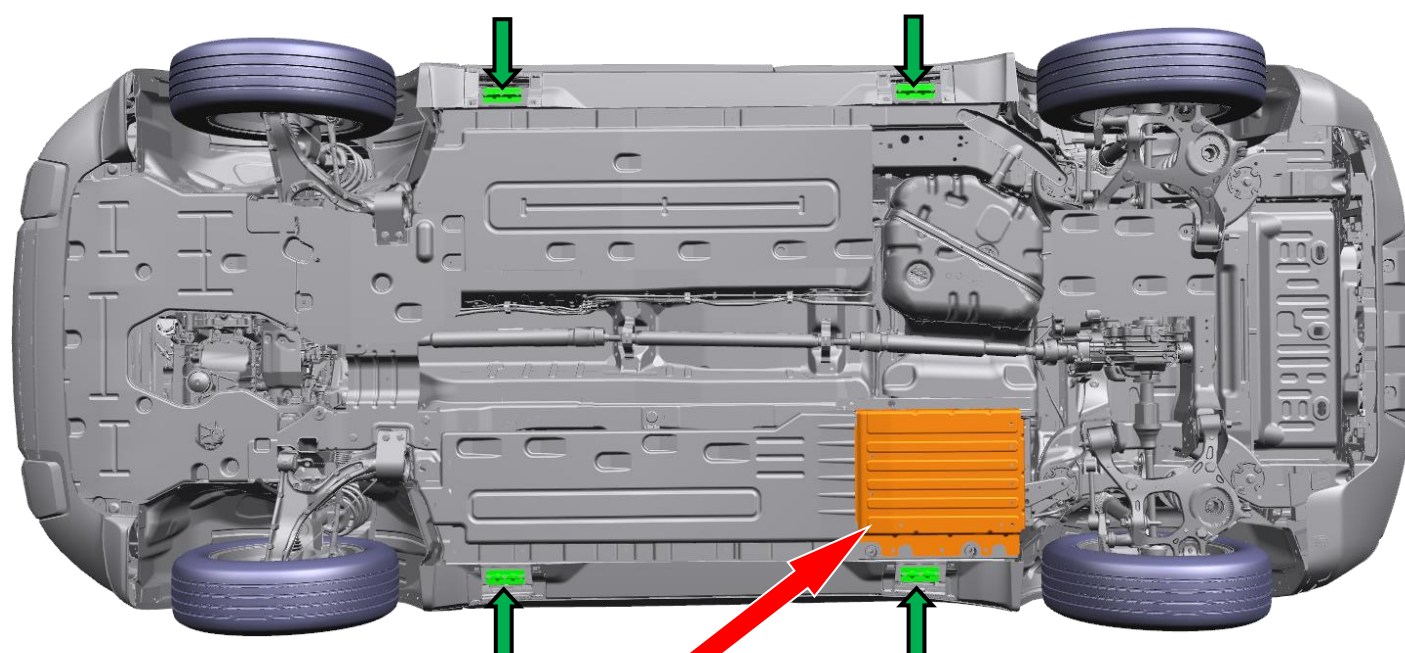
UNDERBODY VIEW
