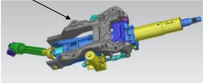
Steering Wheel and Steering Column Mount-Magnesium Alloy
